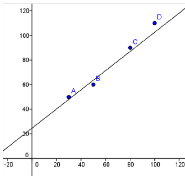
Figura 4.6: Reta S = 24,69388 + 0,78231 \cdot t
