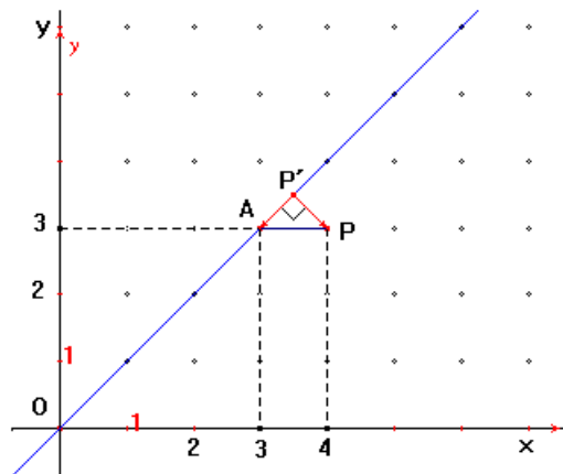
Figura 4.2: P = (4, 3)
