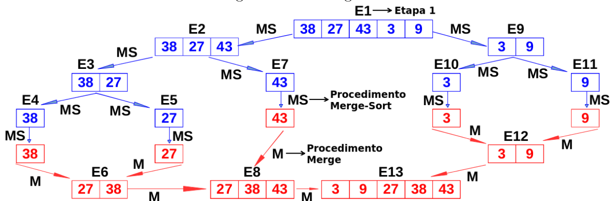
Figura 4.2.1: Merge-Sort
