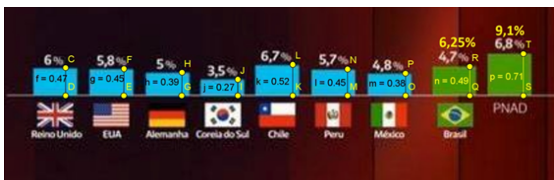
Figura 34 – As colunas mensuradas no GeoGebra.
