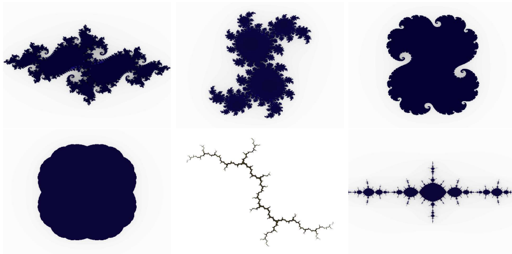
Figura 1: Conjunto de Julia preenchido:(a) c = -0.74 + 0.12i (b) c = 0.37 - 0.28i (c) c = 0.27 + 0.01i (d) c = 0.15 (e) c = i (f) c = -1.312
