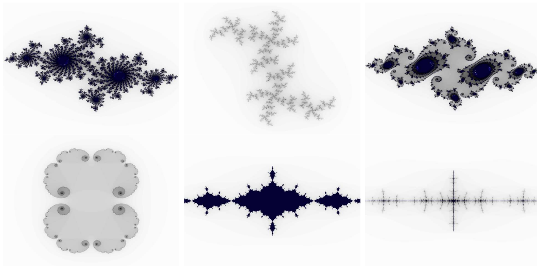
Figura 12: Conjunto de Julia preenchido: (a) c = -0.687 + 0.312i (b) c = 0.3 + 0.6i (c) c = -0.75 + 0.1i (d) c = 0.275 (e) c = -1.2 (f) c = -1.4
