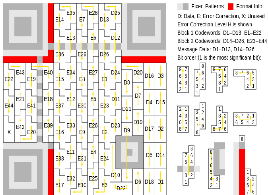
Figura 4: Estrutura do QR Code Fonte: https://en.wikipedia.org/wiki/QR_code#Structure – head
