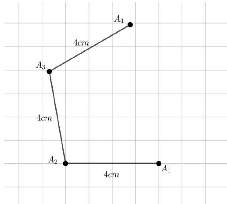
Figura 20 – Poligonal A_1A_2A_3A_4 .
